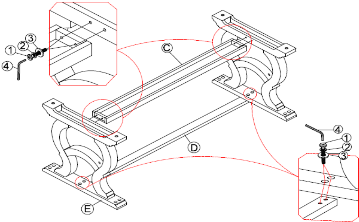
BOTTOM VIEW
