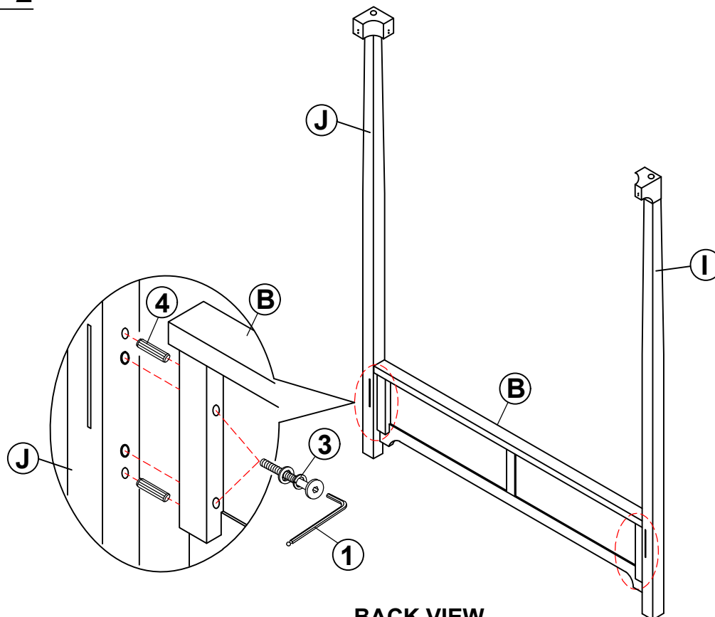
BACK VIEW
