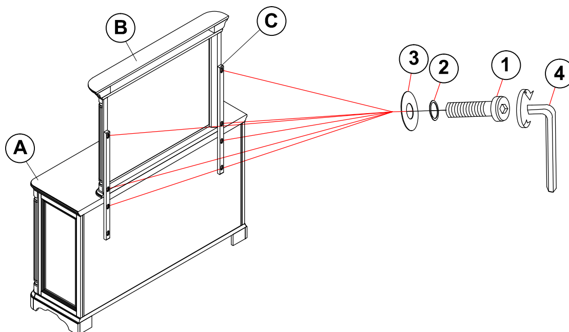
BACK VIEW
