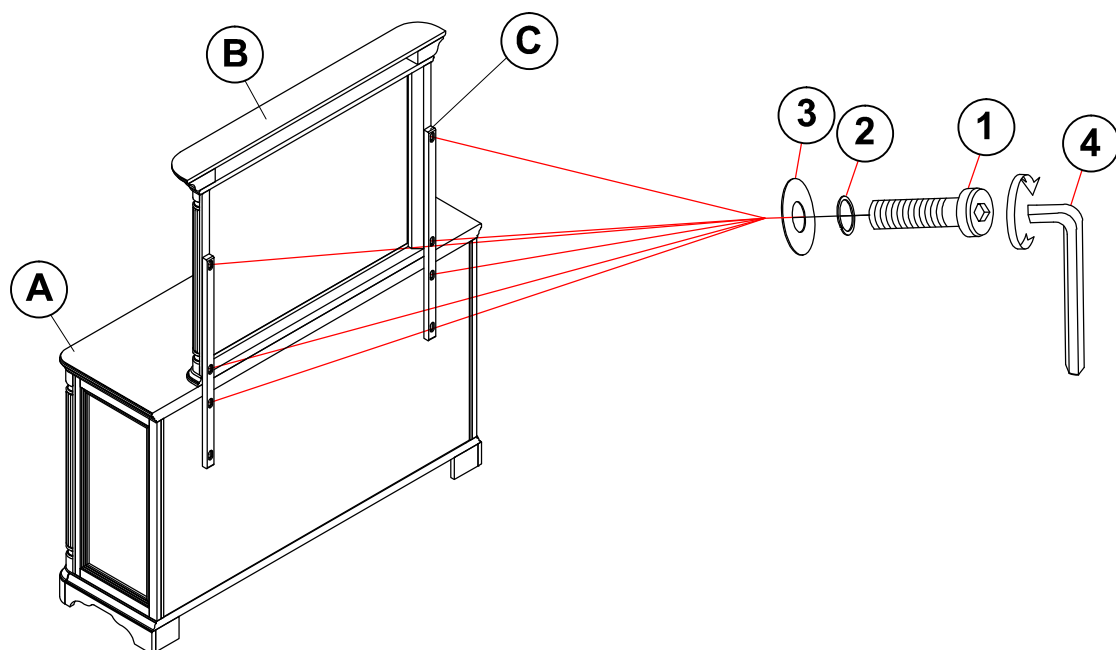
BACK VIEW
