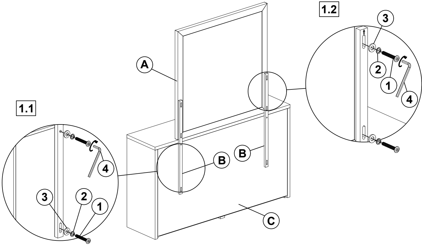
** BACK VIEW
