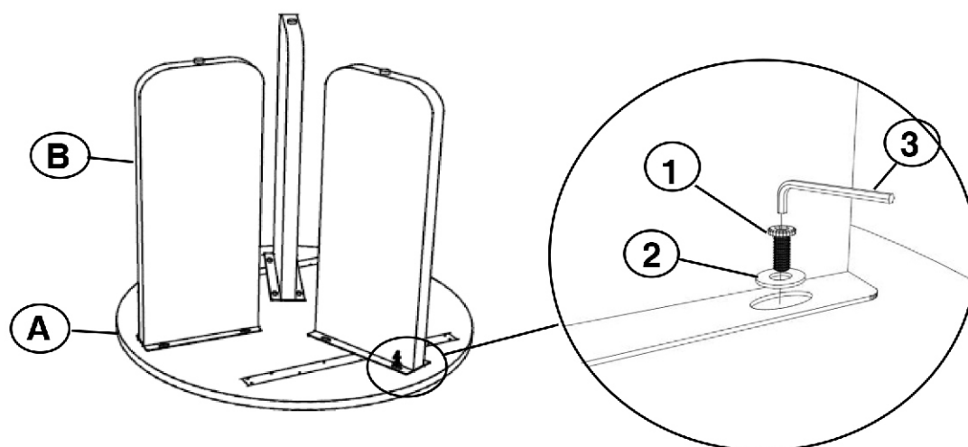
BOTTOM VIEW
