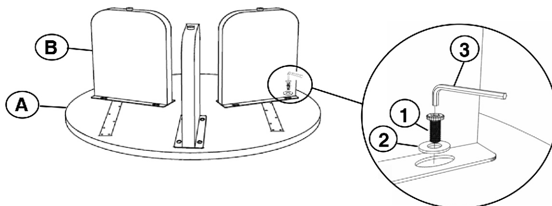
BOTTOM VIEW
